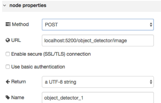
Fig. 4. HTTP Requester properties for Object_Detector_1.
