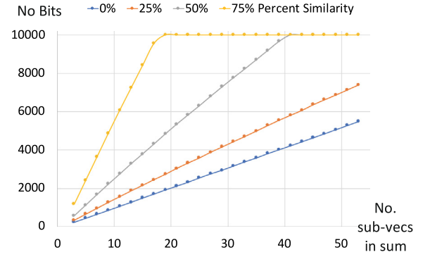
Fig. 8. Minimum message size (No Bits) for chunk vectors containing n sub-feature vectors at differing similarity factors.
