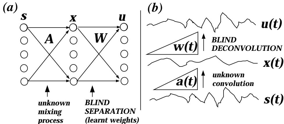
Figure 3: Network architectures for (a) blind separation of 5 mixed signals, and (b) blind deconvolution of a single signal.
