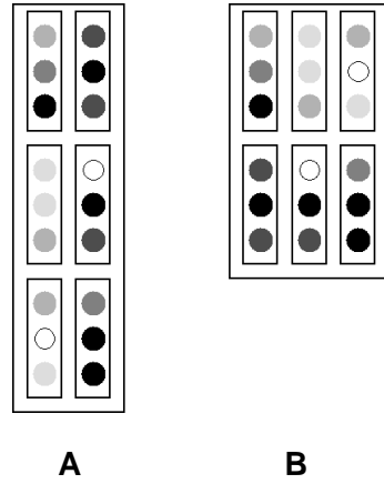
Figure 5: Schematic illustration of the vector transpose (following Marimont & Wandell, 1992). For a matrix \mathbf{Y} considered as a two-dimensional array of stacked vectors (A), its vector-transpose \mathbf{Y}^{\text{VT}} is defined to be the same stacked vectors with their row and column positions in the array transposed (B).
