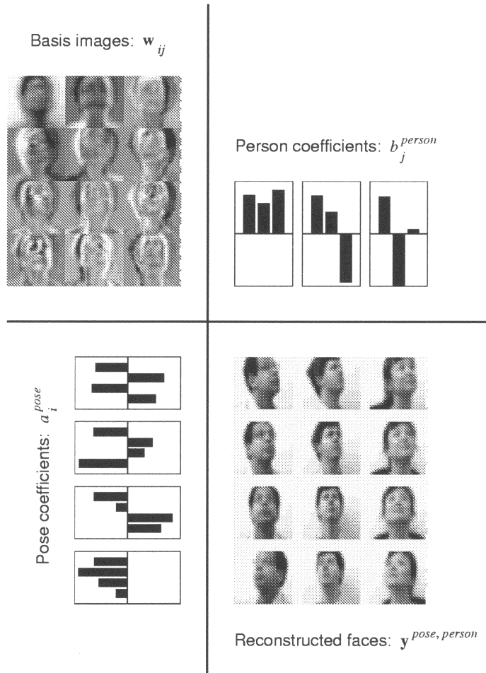
Figure 2: Illustration of a symmetric bilinear model for a small set of faces (a subset of Figure 6). The two factors for this example are person and pose. One vector of coefficients, a_i^{pose} , describes the pose, and a second vector, b_j^{person} , describes the person. To render a particular person under a particular pose, the vectors a_i^{pose} and b_j^{person} multiply along the four rows and three columns of the array of basis images w_{ij} . The weighted sum of basis images yields the reconstructed faces y^{pose, person} .
