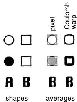
Figure 8: The result of averaging shapes together under different representations. Averaging in a pixel representation always gives a “double exposure” of the two shapes. Under the Coulomb warp representation, a circle averaged with a square gives a rounded square; a filled circle averaged with a square gives a very thick rounded square. The letter A averaged with the letter B yields a shape that is arguably intermediate to the shapes of the two letters. This property of the representation makes it well suited to linear algebraic manipulations with bilinear models.
