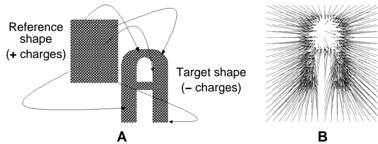
Figure 7: Coulomb warp representation for shape. A target shape is represented by the displacements that a collection of ink particles would undergo to assemble themselves into the target shape. (A) Correspondences between ink particles of the reference shape and those of the target shape are found by tracing the electrostatic force lines between positively and negatively charged ink particles. (B) The vector from the start to the end of the field line specifies the translation for each particle. The result is a smooth warp, with similar shapes represented by similar warps.
