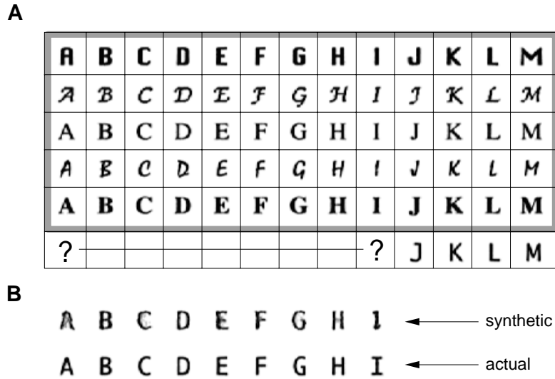
Figure 9: Style extrapolation in typography. (A) Rows 1–5: The first 13 (of 62) letters of the training fonts. Row 6: The novel test font, with A–I unseen by the model. (B) Row 1: Font extrapolation results. Row 2: The actual unseen letters of the test font.
